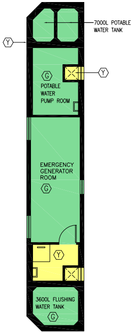
MECHANICAL FLOOR (AT LEVEL 106.45)
