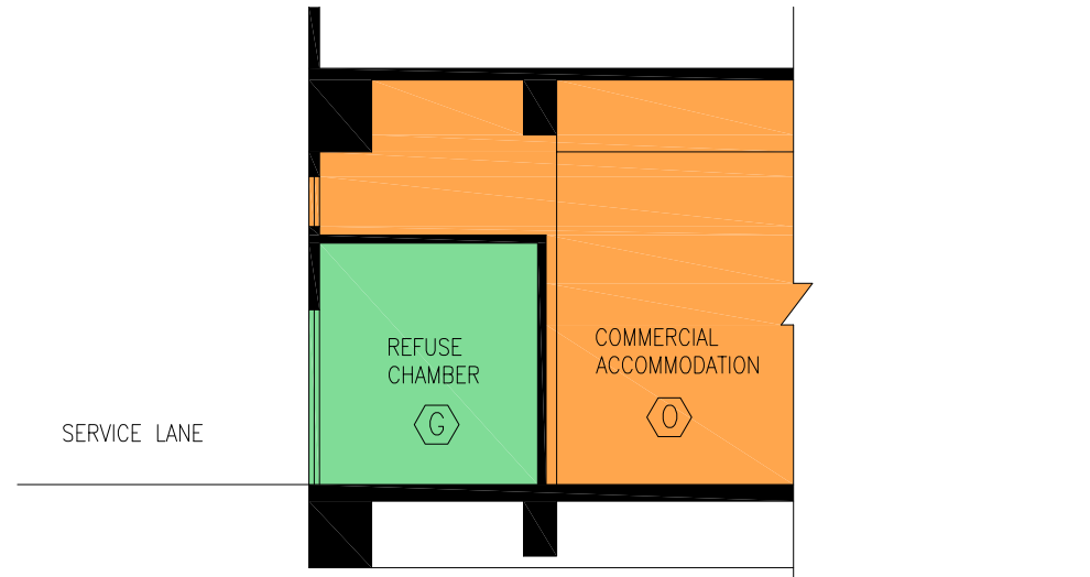
SECTION 'X' FOR REFUSE CHAMBER AT GROUND FLOOR
