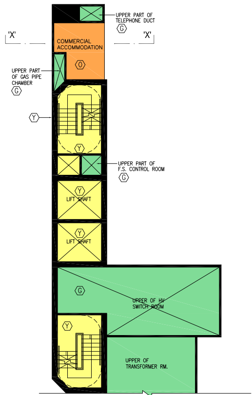
PART PLAN BETWEEN G/F & 1/F
